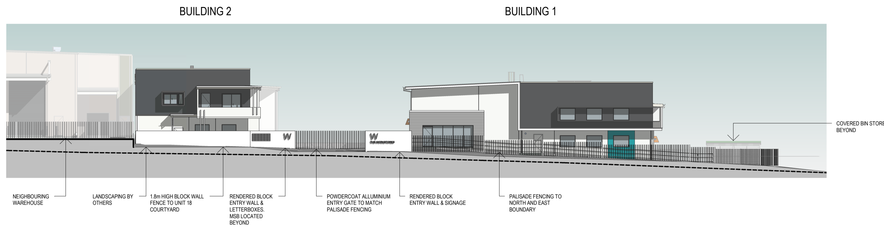
2 LOT 1 EAST ELEVATION 1: 250
